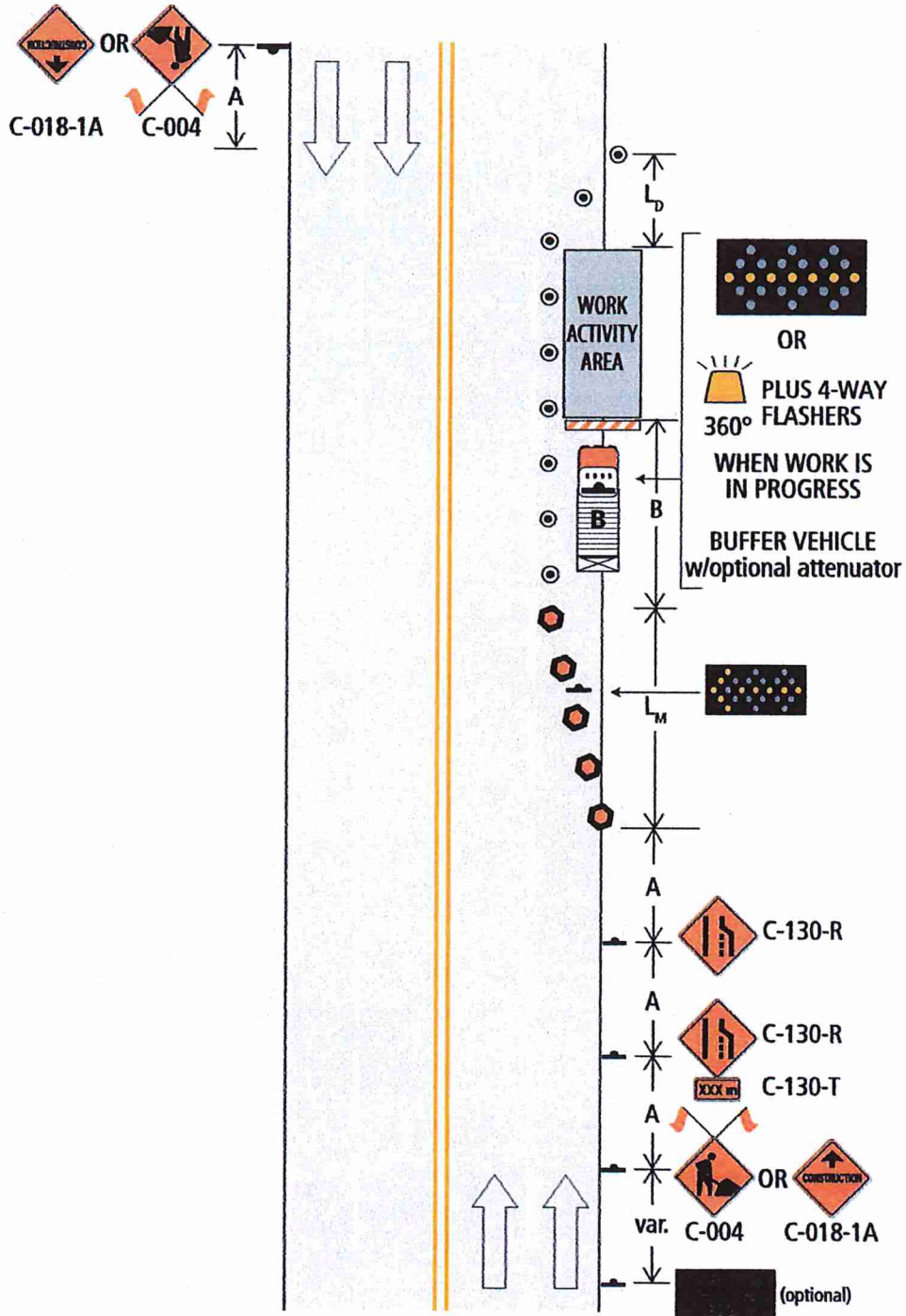
Figure 8.6: Right Lane Closed – Short and Long Duration
